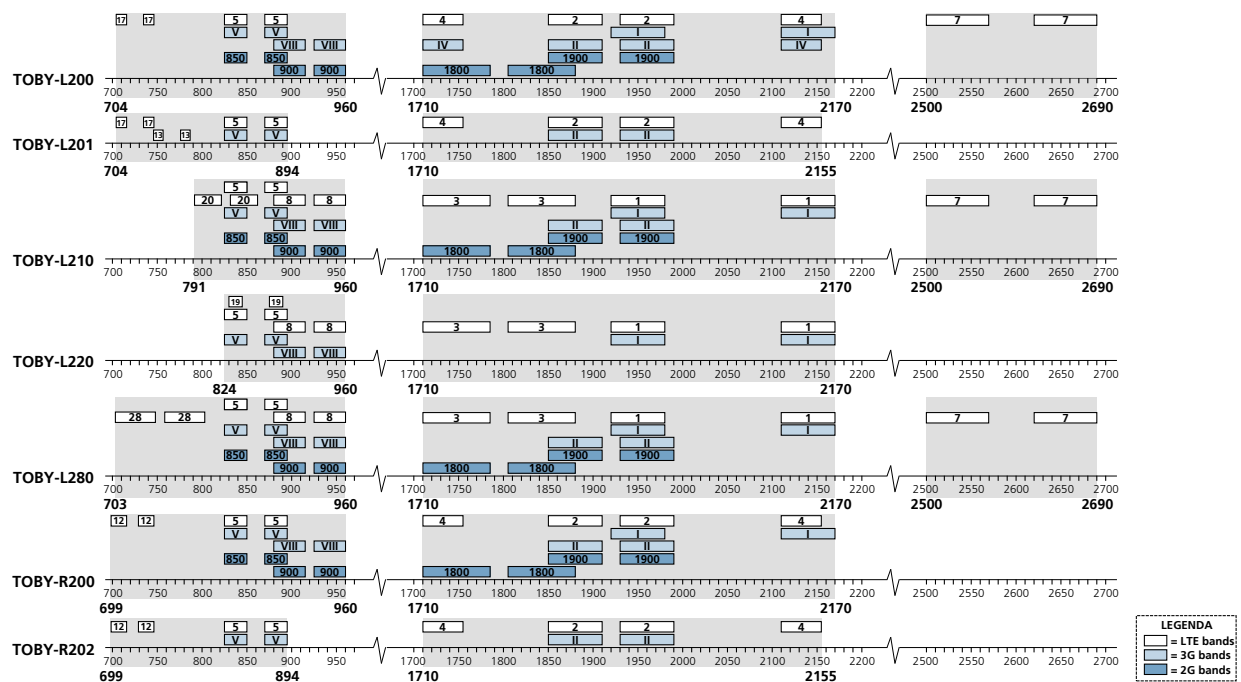
Figure 74: Summary of TOBY-L2 and TOBY-R2 series modules LTE, 3G and 2G operating frequency bands
