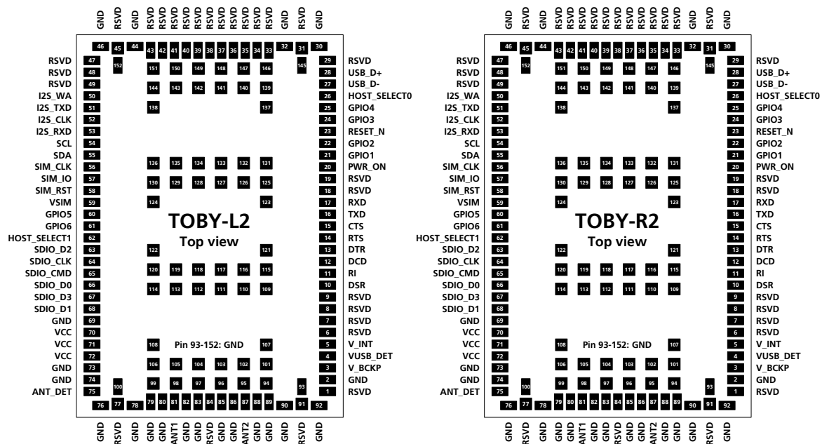
Figure 72: TOBY-L2 and TOBY-R2 series modules pad layout and pin assignment
