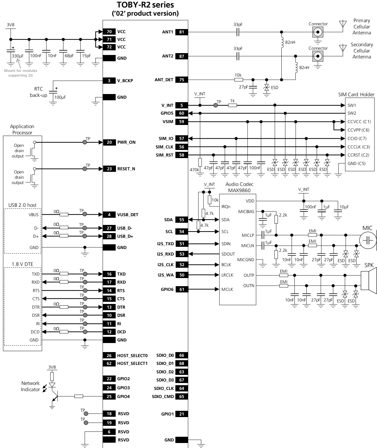
Figure 68: Example of schematic diagram to integrate a TOBY-R2 module "02" product version using all available interfaces
