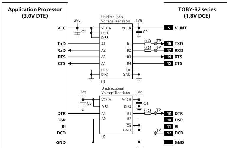
Figure 53: UART interface application circuit with partial V.24 link (6-wire) in DTE/DCE serial communication (3.0 V DTE)
