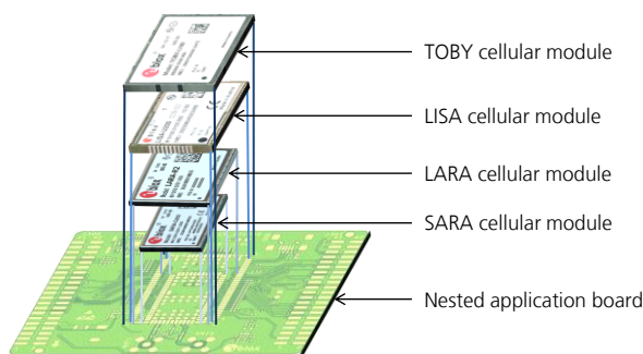
Figure 73: TOBY, LISA, SARA, LARA modules' layout compatibility: all modules are accommodated on the same nested footprint
