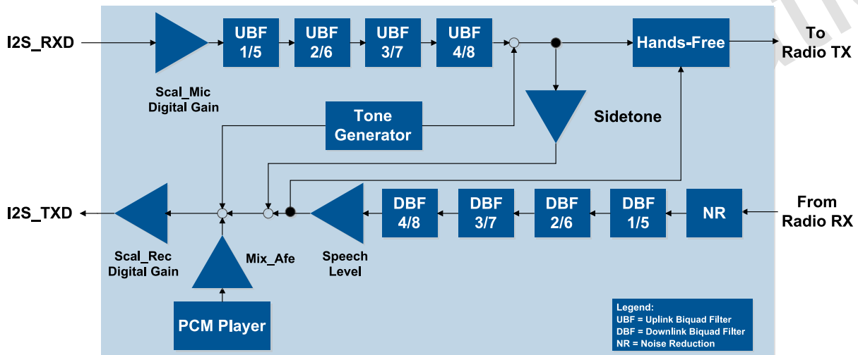
Figure 13: Audio paths
