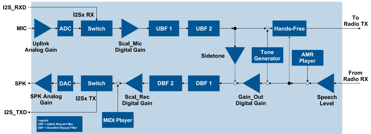
Figure 16: Audio paths
