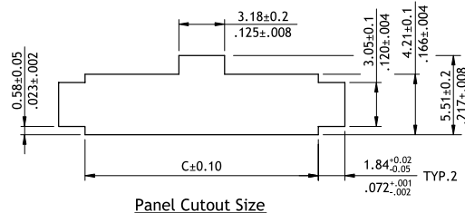
Panel Cutout Size
